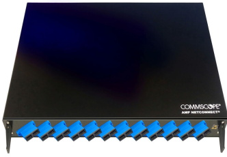
FMS Fiber Optic Termination Panel, 1U, 19 in, 24 SC/UPC, singlemode, OS2, black
